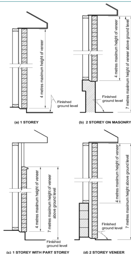
Figure 9.2.3.1: Masonry veneer height limitations Paragraph 9.2.3.1
